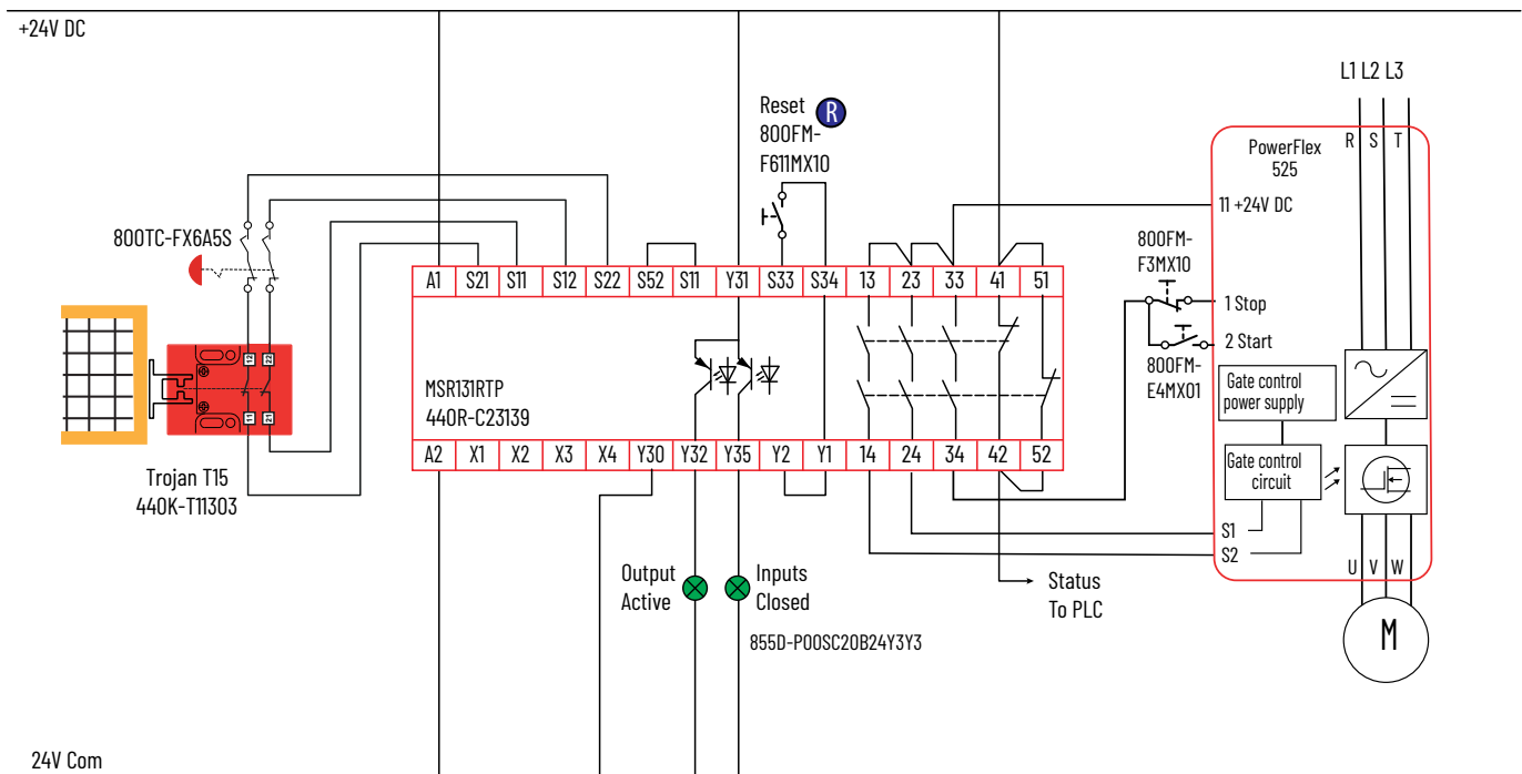
Figure 31 - MSR131RTP with Trojan T15 and 800T E-stop
