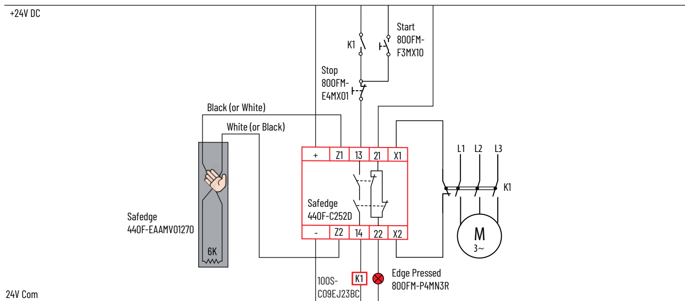
Figure 42 - Safedge Single Channel, Automatic Reset
