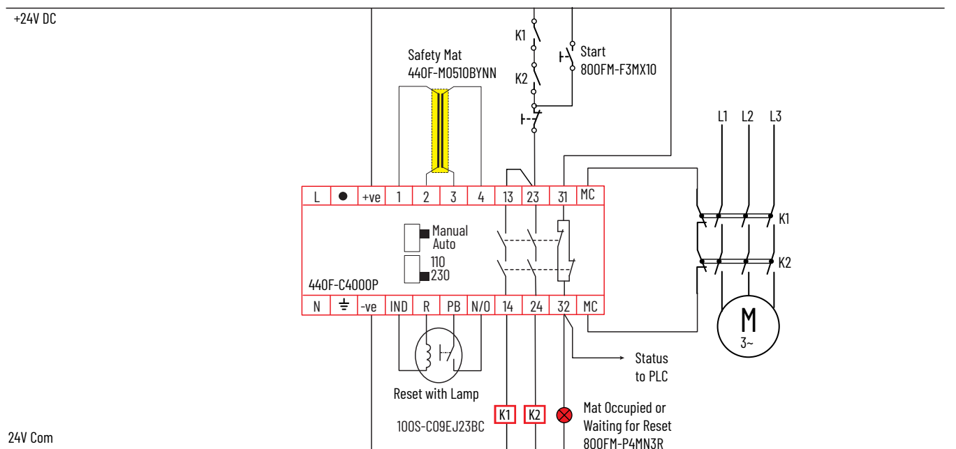
Figure 39 - 440F-C4000P with 440F Safety Mat
