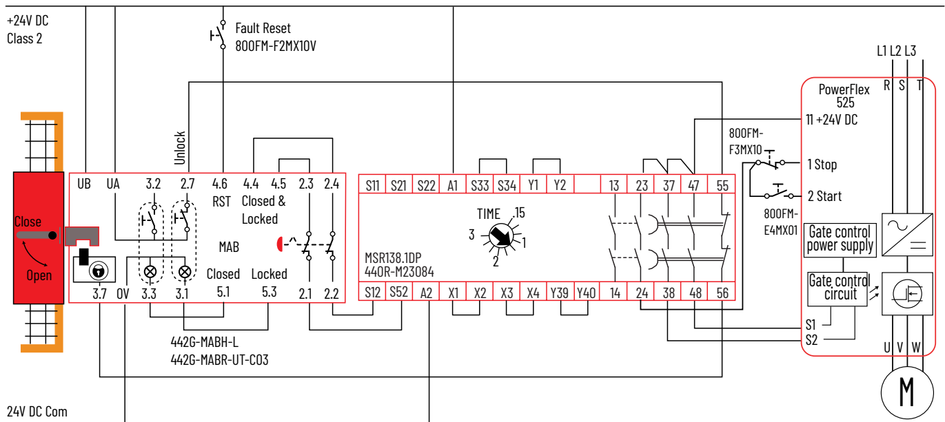
Figure 34 - MSR138.1DP Safety Relay with MAB (Integral Buttons)
