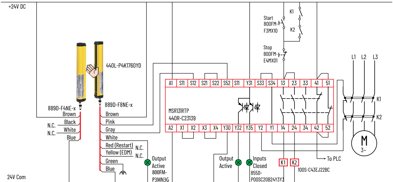
Figure 30 - MSR131 with 440L Safety Light Curtain
