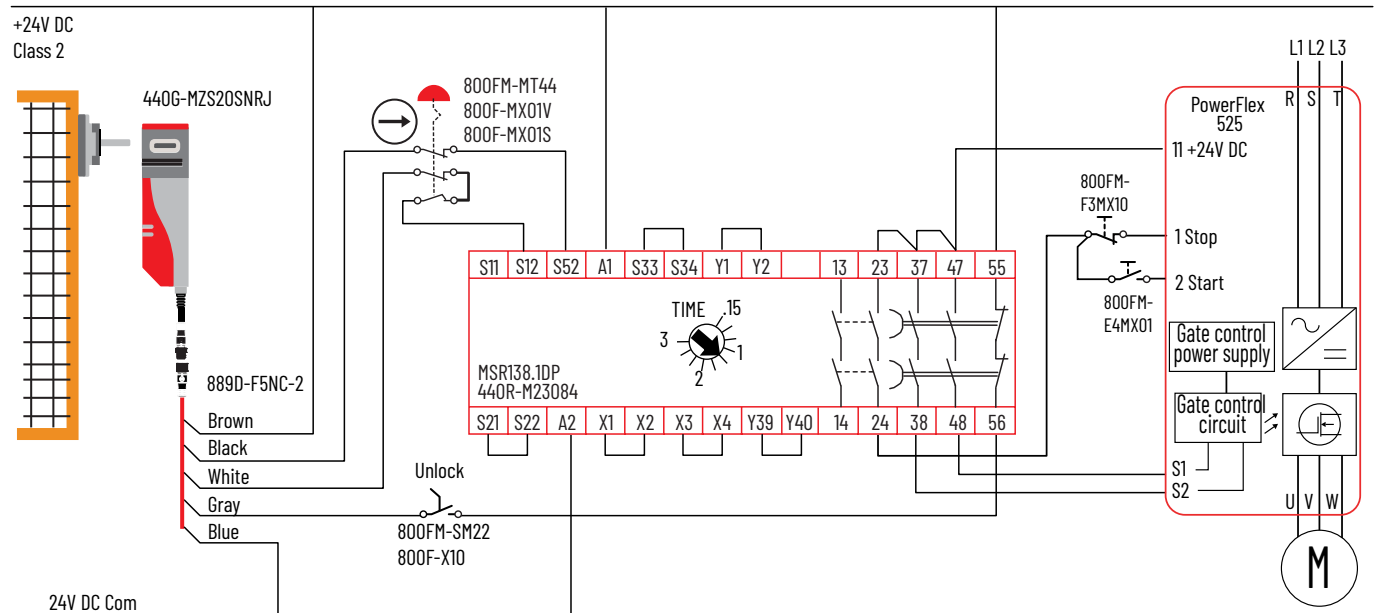
Figure 35 - MSR138.1DP Safety Relay with 440G-MZ and 800F E-stop
