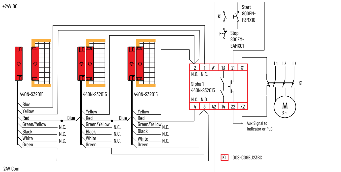
Figure 44 - Sipa 1 with Sipa Sensors
