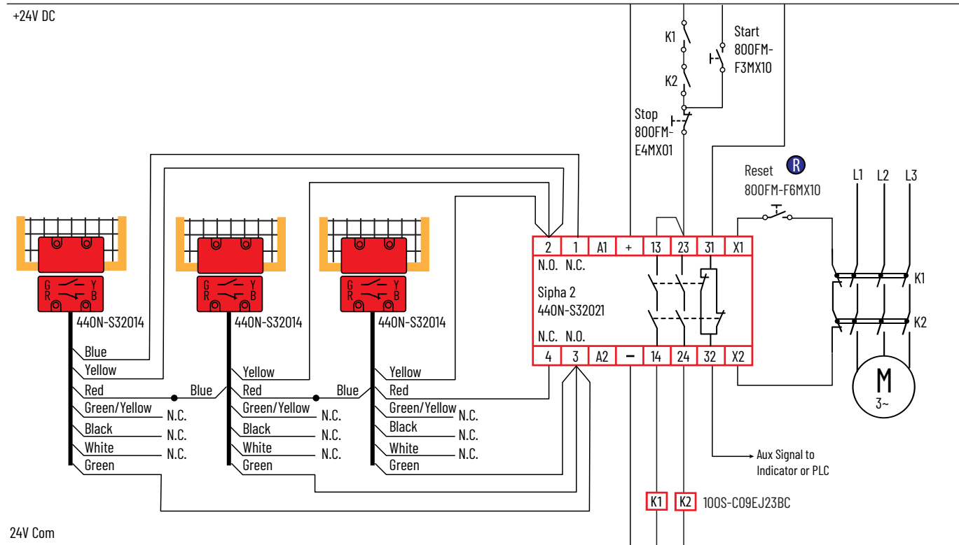
Figure 43 - Sipa 2 with Series Connection of Sensors
