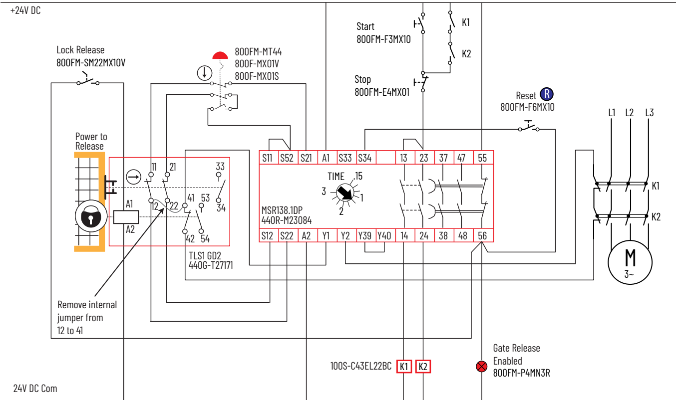
Figure 32 - MSR138.1DP Safety Relay with TLS1-GD2 Switch and 800F E-stop
