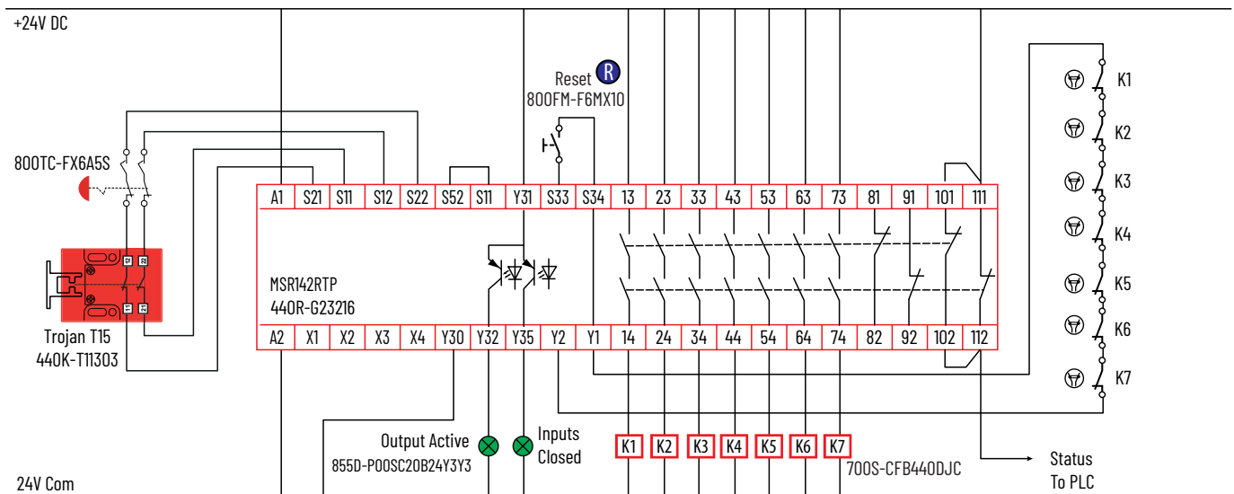
Figure 37 – MSR142 with 440K Trojan T15 and 800TC E-stop
