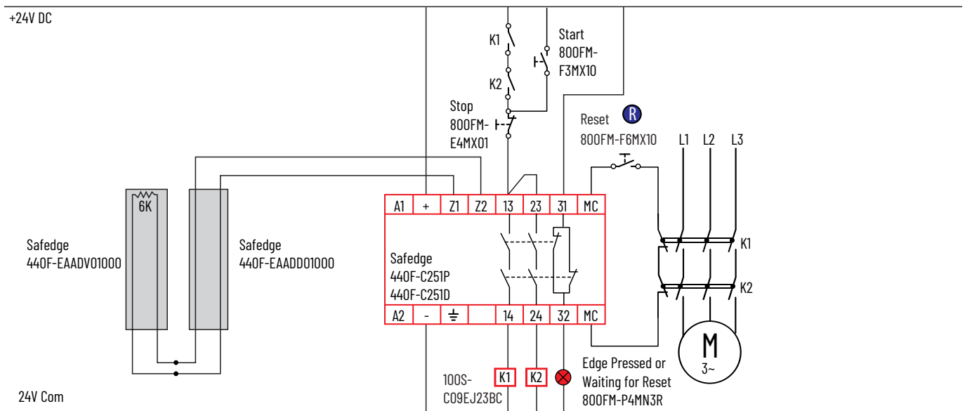
Figure 41 - Safedge Dual Channel
