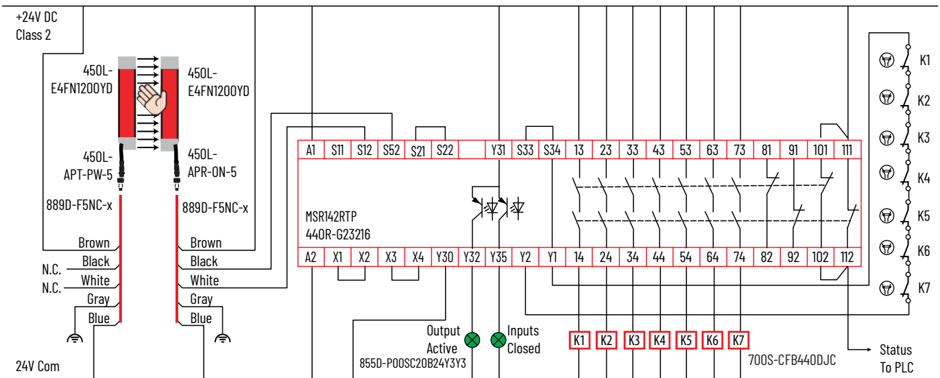
Figure 38 - MSR142 with 450L Safety Light Curtain
