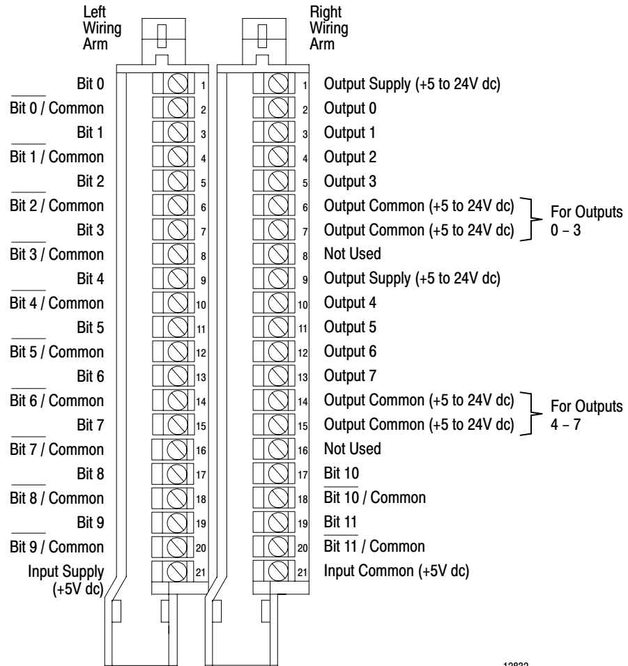
Figure 2.3 Terminal Identification
