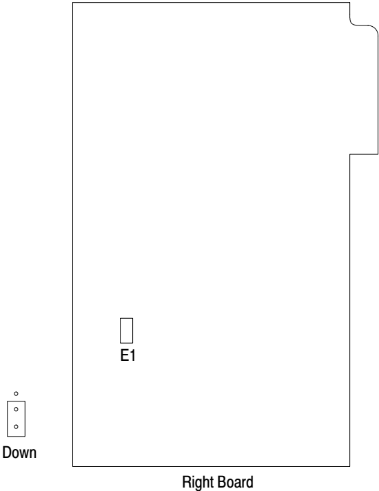
Figure 3.2 Configuration Plug Location and Settings (Right Board)
