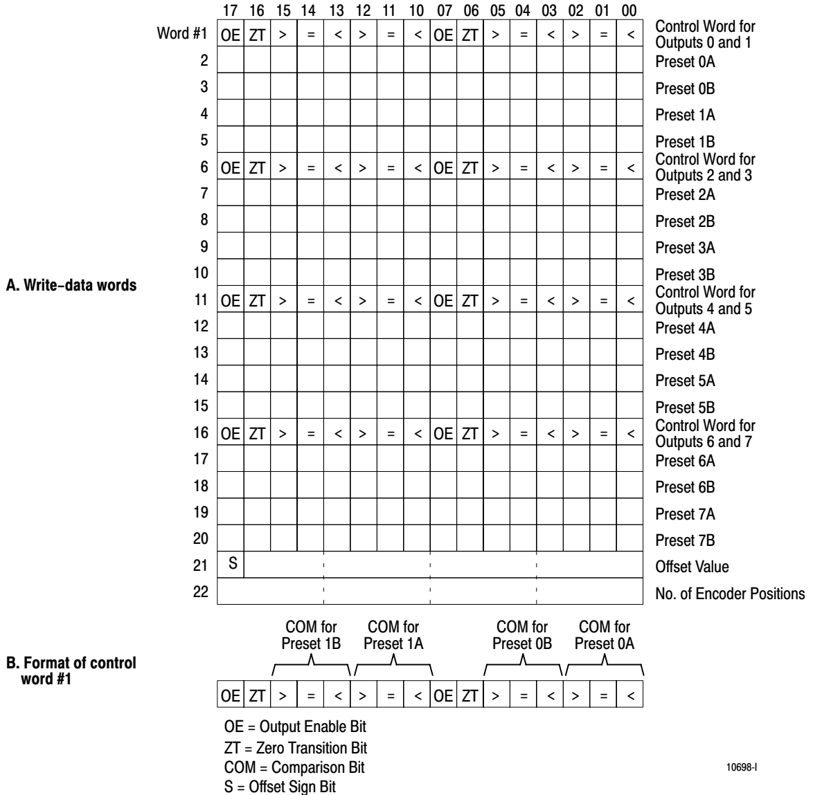
Figure 5.1 Format of Block-transfer-write Data with Offset
