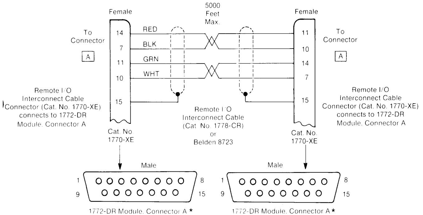
Figure 9 Remote I/O interconnect cable (Cat. No. 1778-CR) and connectors (Cat. No. 1770-XE) for connection of line driver receiver modules
