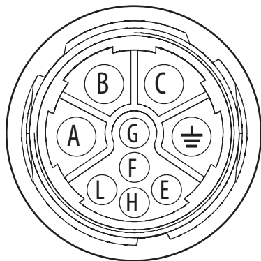
M23 Motor Connector Pinouts
