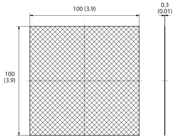
Figure 2 - Dimensions (mm [in.])
