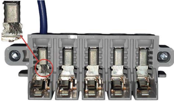
Figure 2 - Proper Wire Insertion
