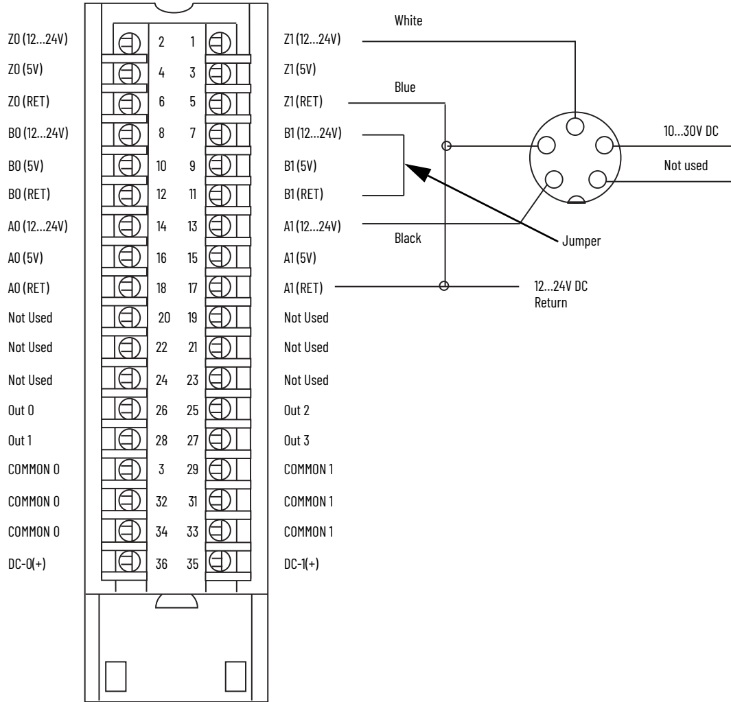
PHOTOSWITCH Series 10,000 Photoelectric Sensor
