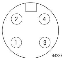
Mini-style 4-Pin Male Receptacle (on the ArmorBlock)
