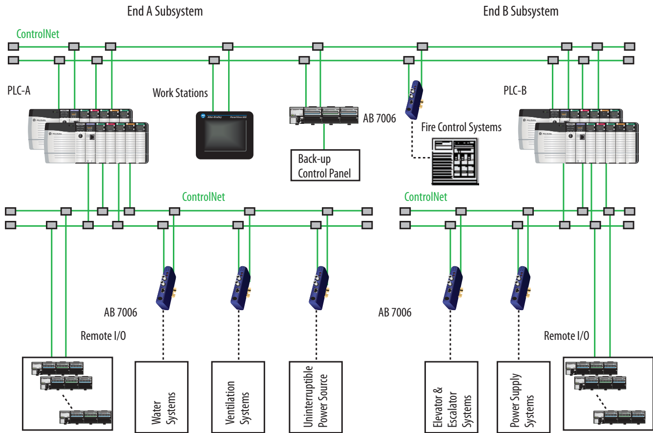
BAS system Diagram for Basic Metro System
