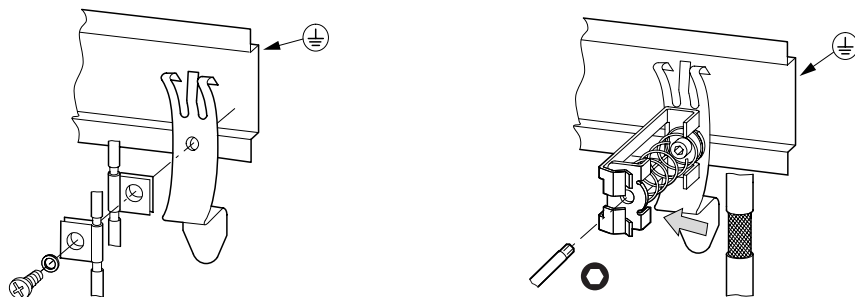
Figure 1.3 Shield Connection to the Mounting Rail
