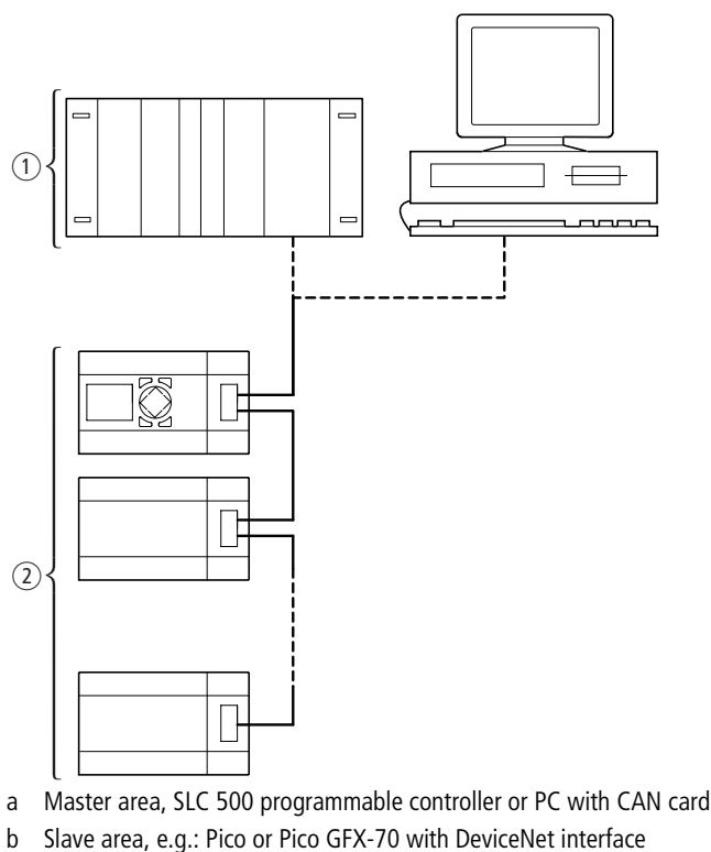
Figure 1.1 Implementation of 1760-DNET in DeviceNet
