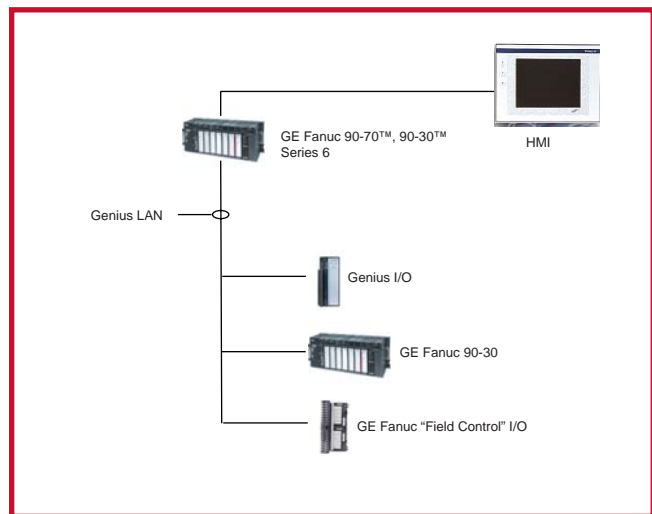
Legacy System
