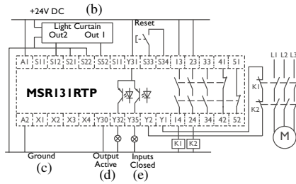
(f) Light Curtain, Monitored Manual Reset, Monitored Output
