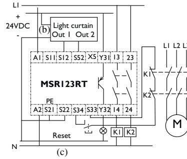
(d) 115/230V Supply, 24V DC Light Curtain, Monitored Manual Reset, Monitored Output
