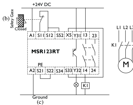
(d) Single Channel Safety Gate, Automatic Reset, No Output Monitoring
