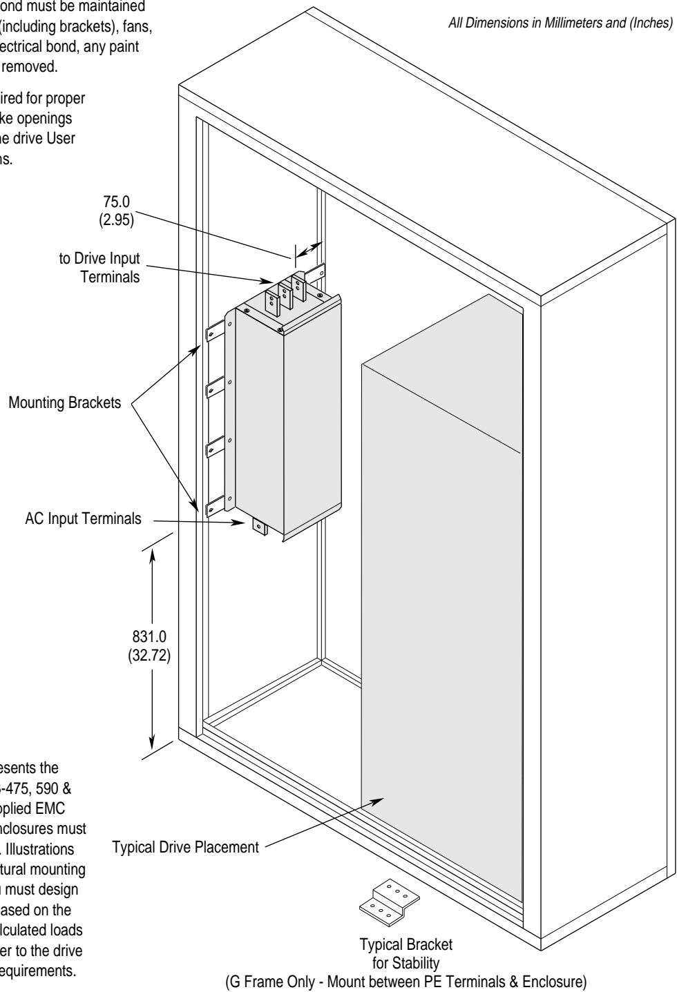
Figure 5 1336 PLUS, PLUS II, FORCE & IMPACT (Typical Filter Mounting) Frames F & G 1, 2
