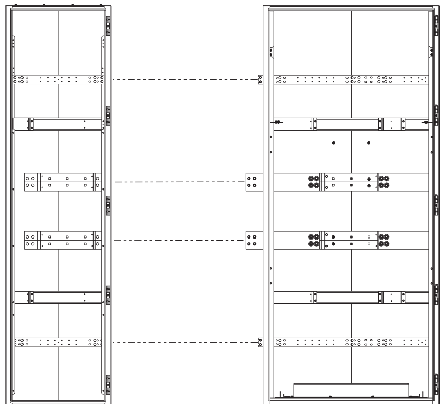
Adjacent Enclosure (Front View) with Bus Bars to be Connected to AFE Right-side Splices
