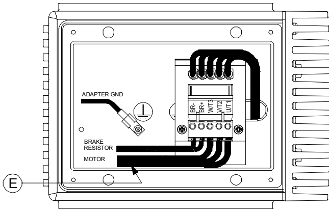
View Z
