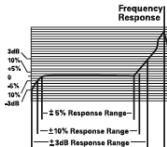
Fig 4 - FREQUENCY RESPONSE CURVE Sensitivity Deviation vs. Frequency
