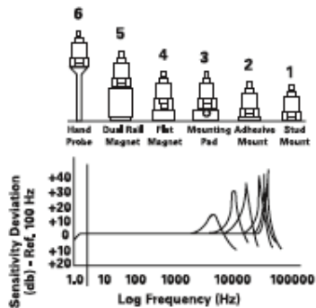
Fig 6 - MOUNTED RESONANCE CHANGE
