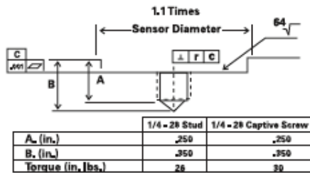
Fig 5 - STUD MOUNTING SURFACE PREPARATION
