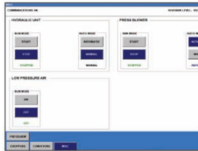
Auxiliaries also Controlled through Graphical Screens
