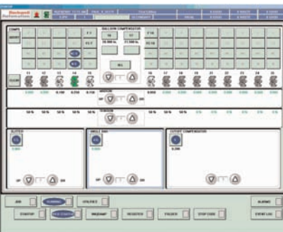
Motor Selection & Monitoring Available for Allen-Bradley Press Drives
